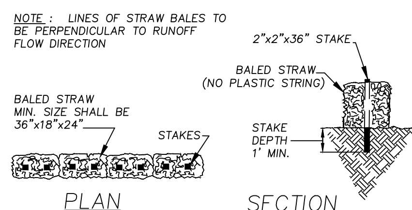
STRAW BALE DIKE NOT TO SCALE
