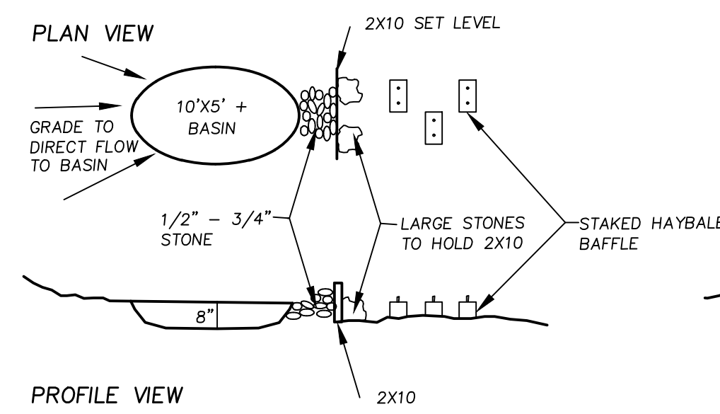
TEMPORARY DEWATERING AREA NOT TO SCALE
