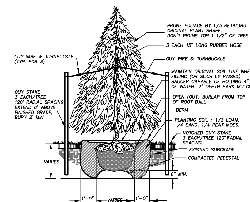
EVERGREEN TREE PLANTING DETAIL
