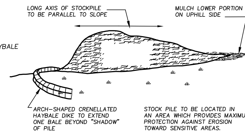
TEMPORARY STOCKPILE NOT TO SCALE
