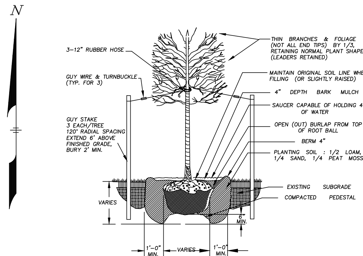
DECIDUOUS TREE PLANTING
