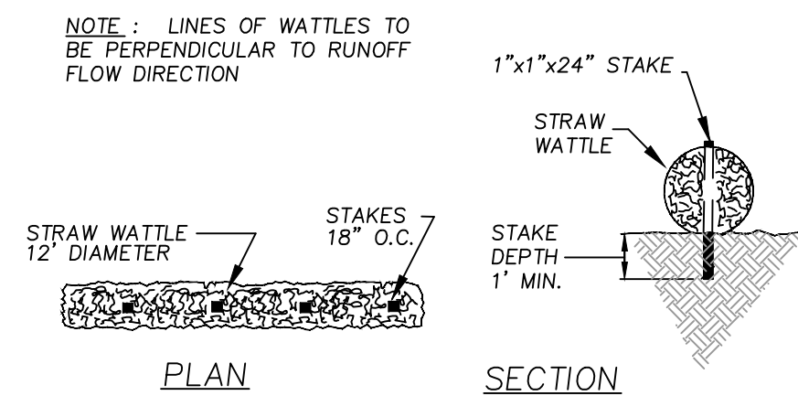
STRAW WADDLES NOT TO SCALE
