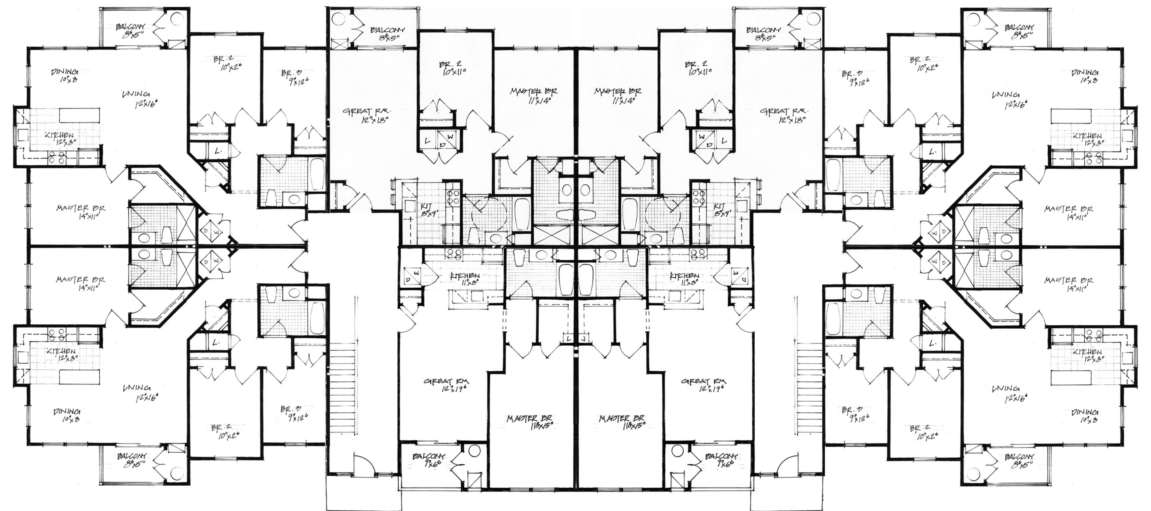
1ST FLOOR PLAN WITH 3 BEDROOM UNITS
